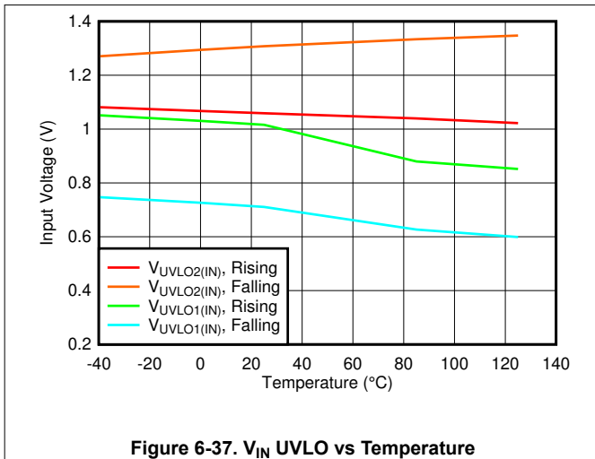
Figure 6-37. V_{IN} UVLO vs Temperature
