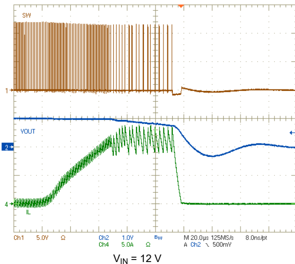
Figure 8-20. Overcurrent Protection – Overload
