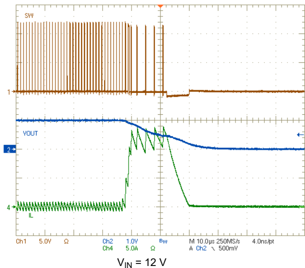
Figure 8-21. Overcurrent Protection – Short
