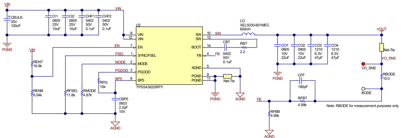
Figure 8-1. 12-V Input, 1.0-V Output, 1-MHz Schematic
