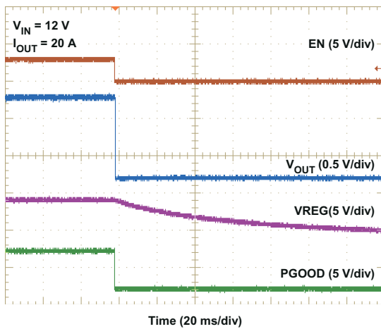
Figure 6-15. Shutdown Waveforms
