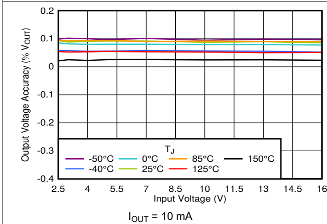
Figure 7-3. V_{OUT} Accuracy vs V_{IN}
