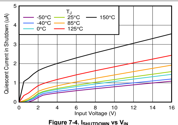
Figure 7-4. I_{SHUTDOWN} vs V_{IN}
