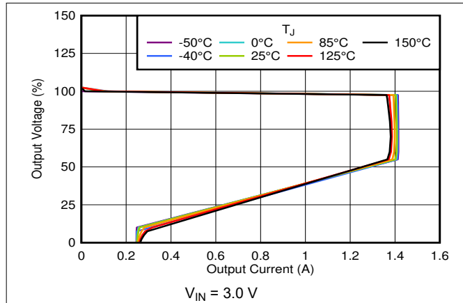
Figure 7-19. Foldback Current Limit vs Temperature
