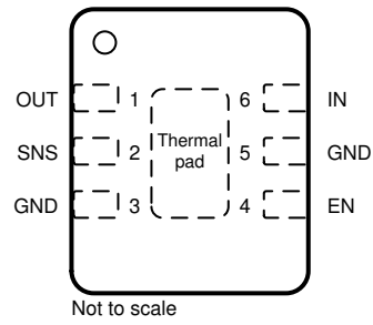
Figure 5-2. DRV Package (Fixed), 6-Pin WSON, Top View
