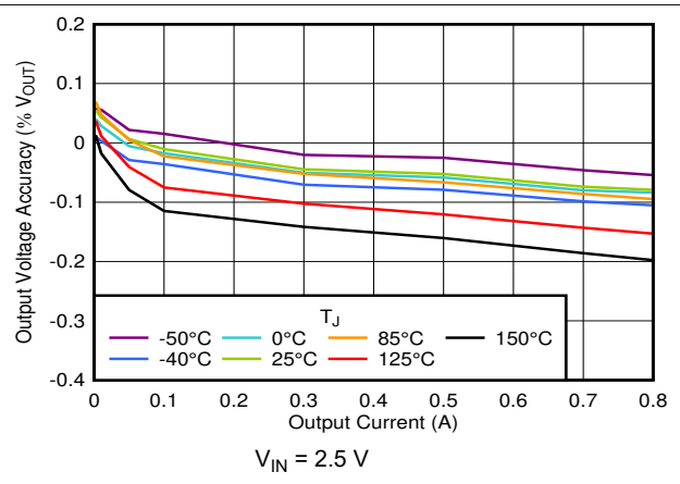
Figure 7-2. V_{OUT} Accuracy vs I_{OUT}
