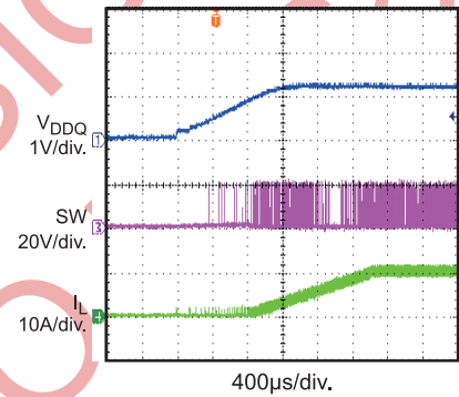
Thermal Recovery I_O = 10A
