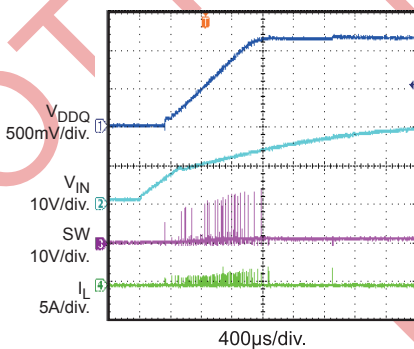
Start up through Vin I_O = 0A
