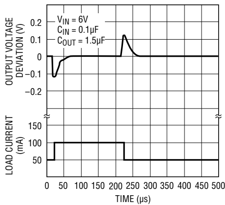
LT1521-5 Transient Response
