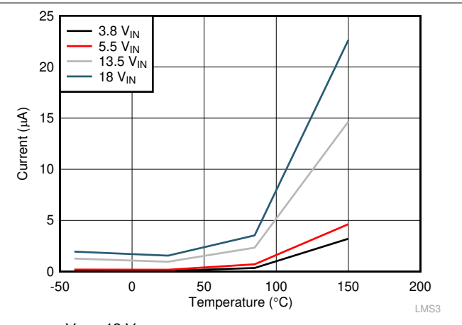
Figure 7-6. Shutdown Current
