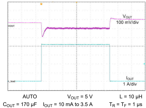
Figure 9-14. Load Transients
