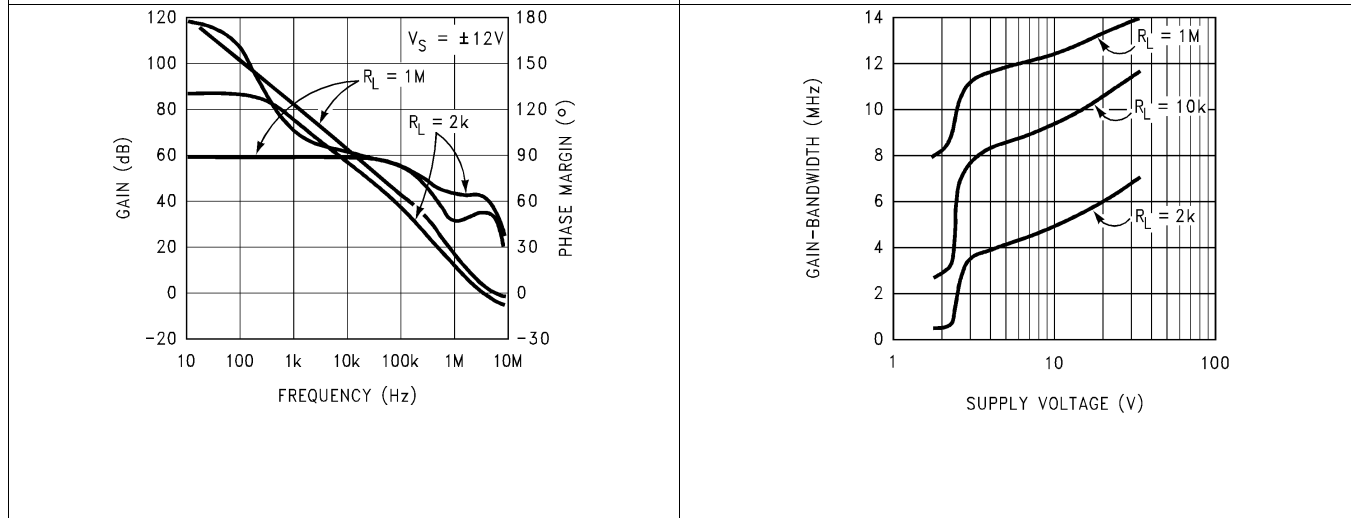
Figure 28. GBW vs. Supply Voltage at 20 kHz
