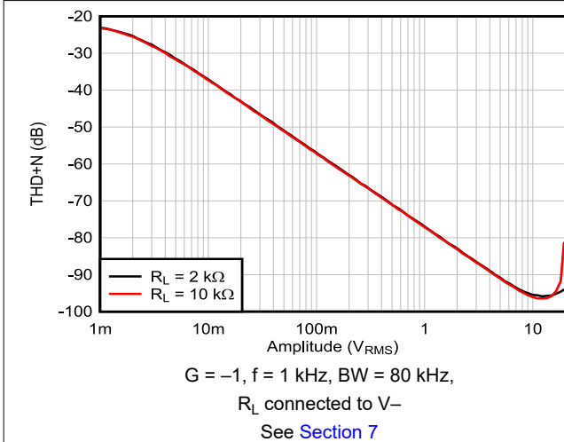
Figure 6-17. THD+N vs Output Amplitude, G = -1
