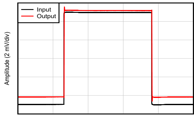
Figure 6-24. Overload Recovery (Positive Rail)
