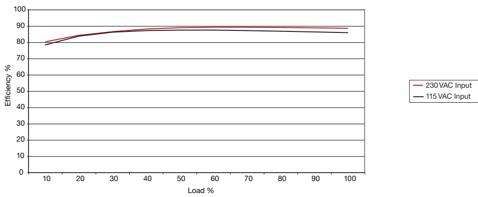
Figure 4 - CCH600PS12
