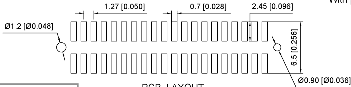
PCB LAYOUT
