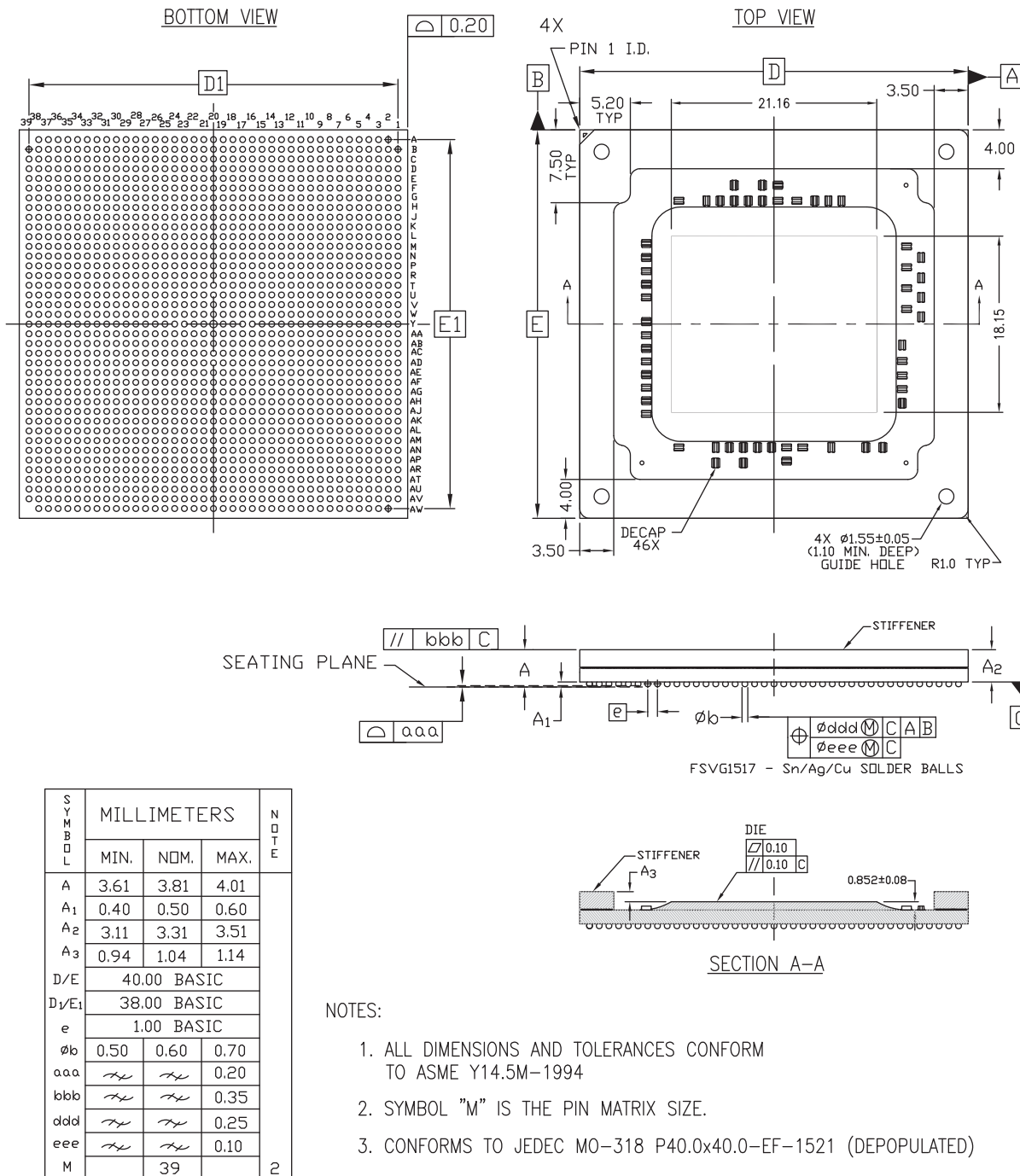
Figure 5-23: Package Dimensions for FSVG1517 (XCZU25DR, XCZU27DR, and XCZU28DR)
