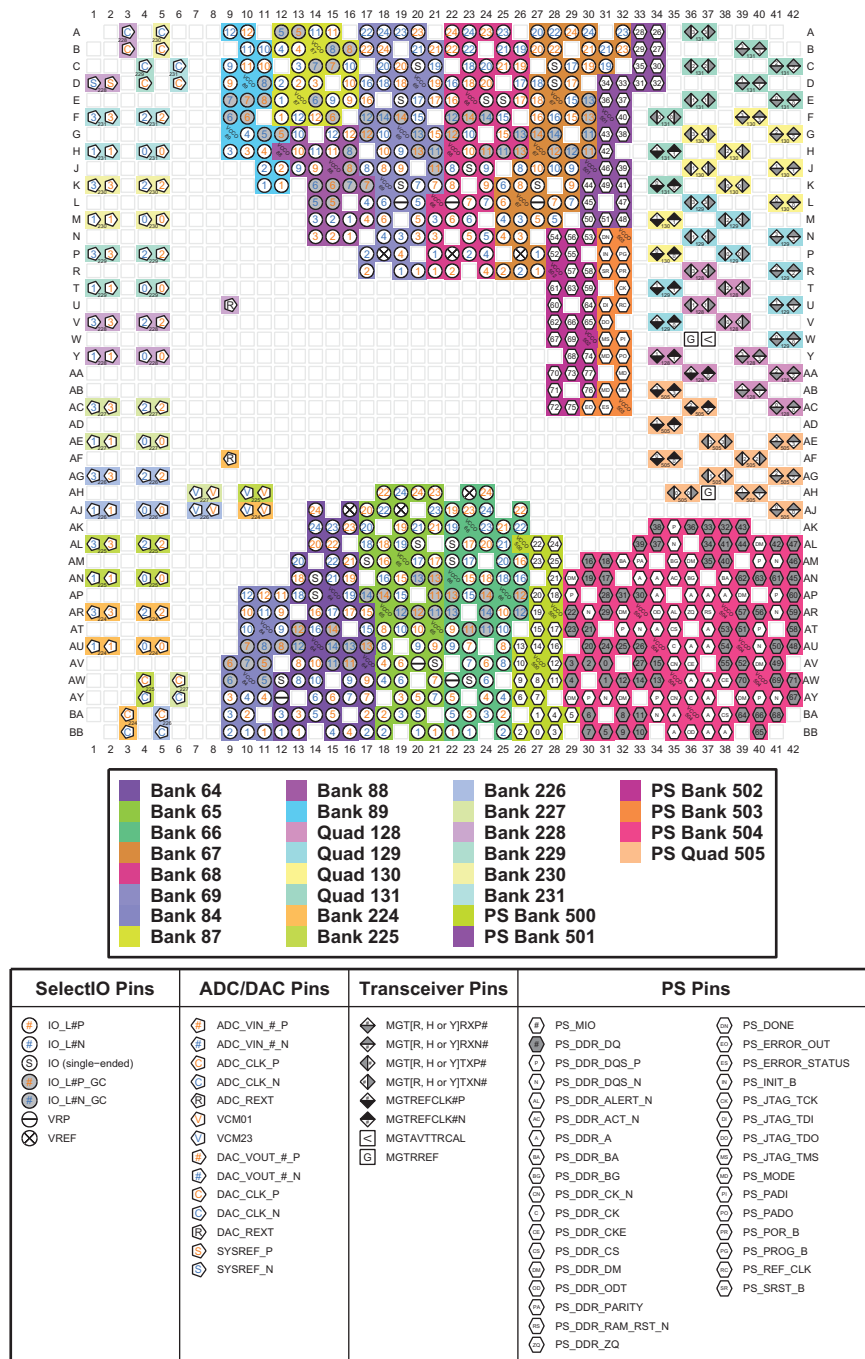
Figure 4-55: FFVF1760 and FSVF1760 Packages—XCZU29DR and XCZU39DR I/O Bank Diagram
