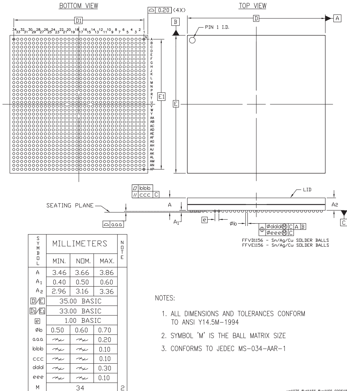
Figure 5-17: Package Dimensions for FFVD1156 (XCZU21DR) and FFVE1156 (XCZU25DR, XCZU27DR, and XCZU28DR)
