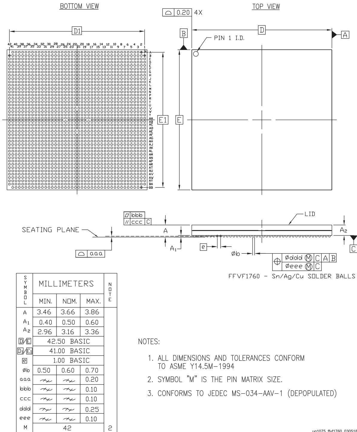
Figure 5-26: Package Dimensions for FFVF1760 (XCZU29DR and XCZU39DR)
