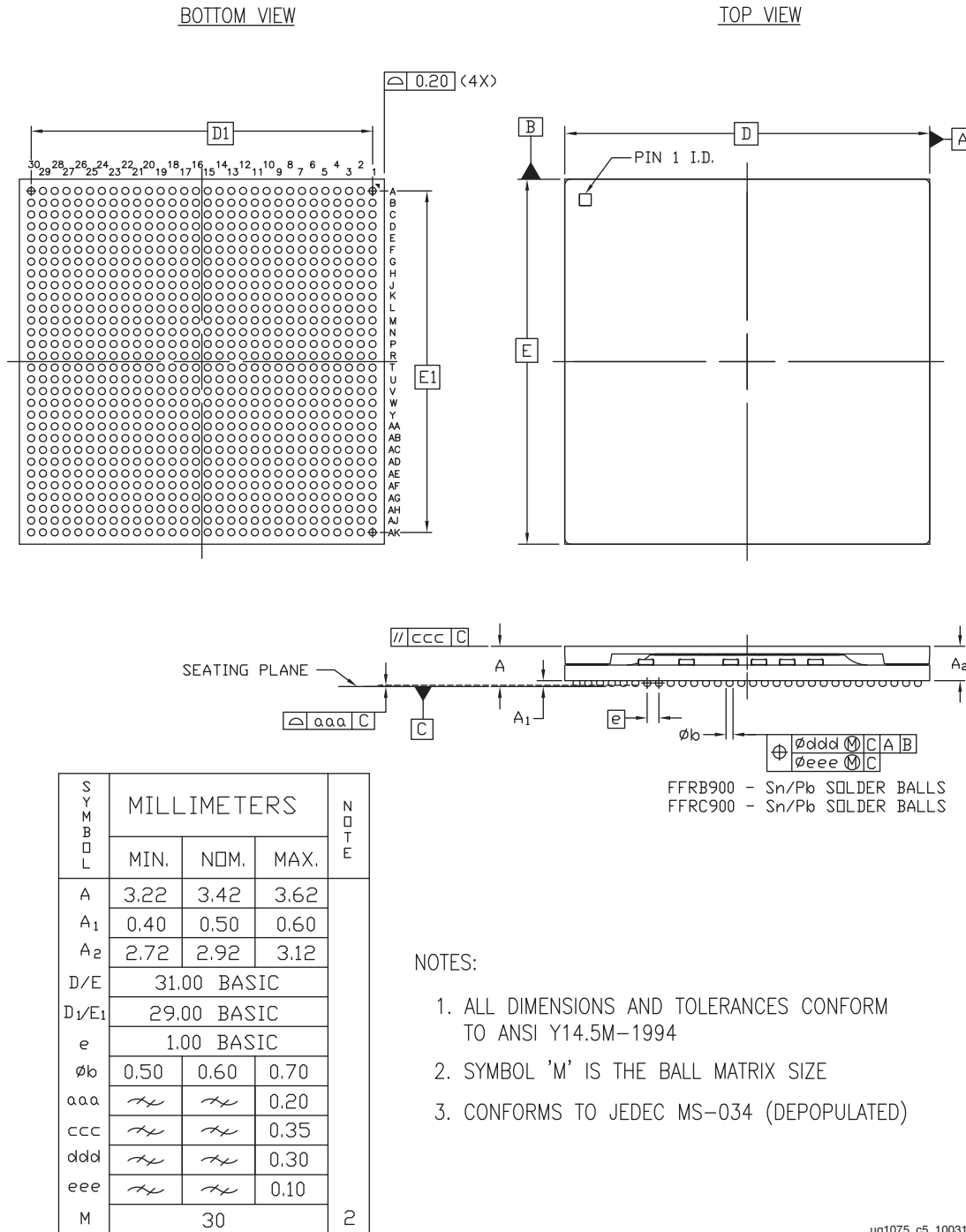
Figure 5-9: Package Dimensions for FFRB900 (XQZU5EV) and FFRC900 (XQZU9EG and XQZU15EG)
