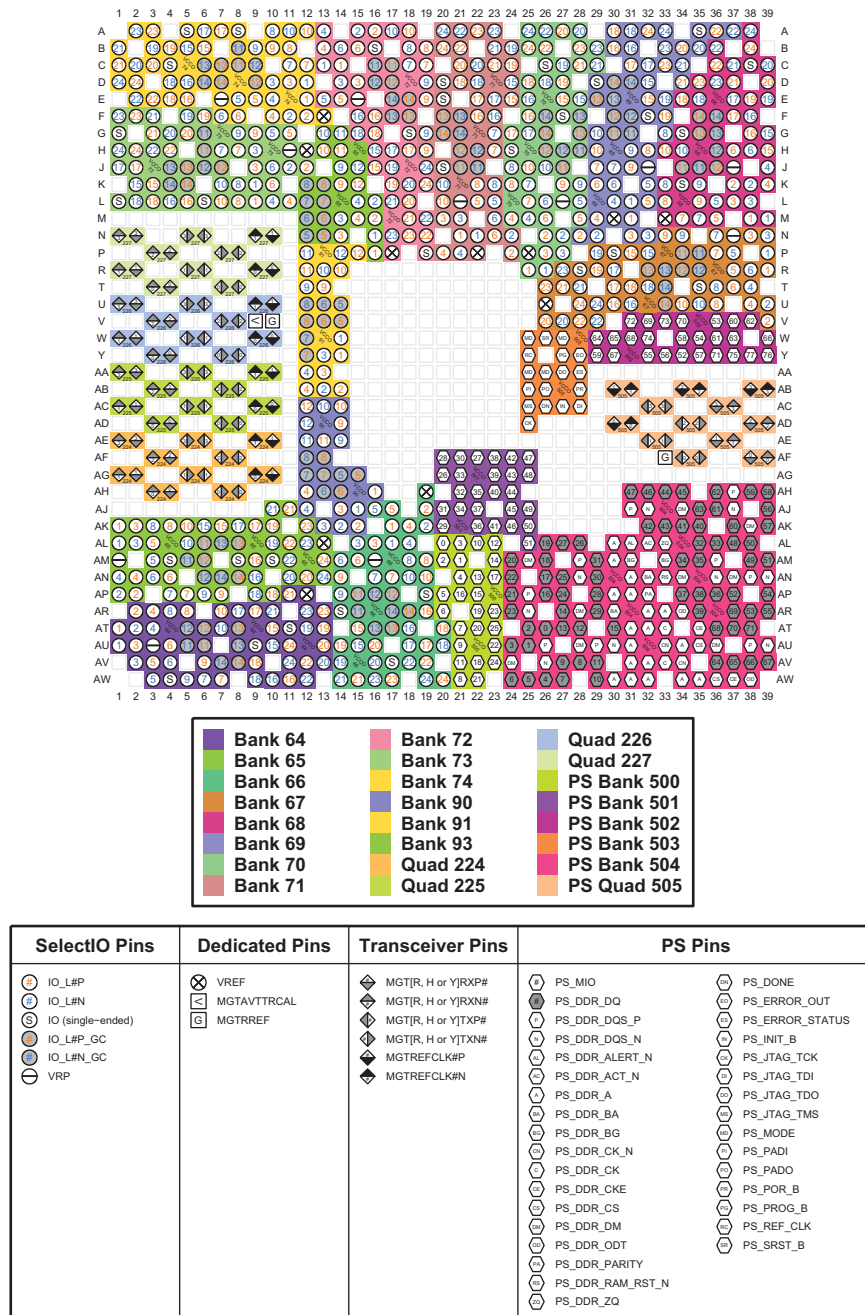
Figure 4-37: FFVB1517 Package—XCZU17EG and XCZU19EG I/O Bank Diagram
