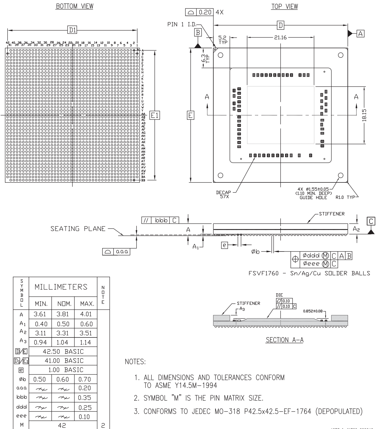
Figure 5-28: Package Dimensions for FSVF1760 (XCZU29DR and XCZU39DR)
