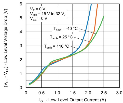
Fig. 12 - Low Level Voltage Drop vs. Low Level Output Current
