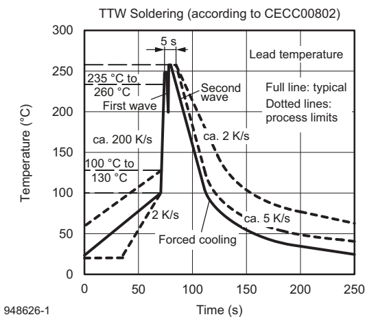
Fig. 22 - Double Wave Soldering of Opto Devices (all Packages)
