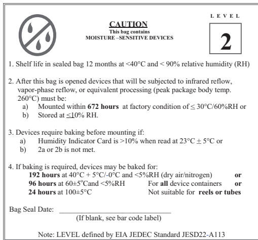
Example of JESD22-A112 level 2 label
