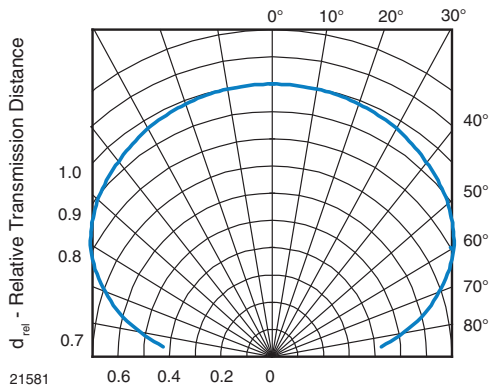
Fig. 11 - Horizontal Directivity
