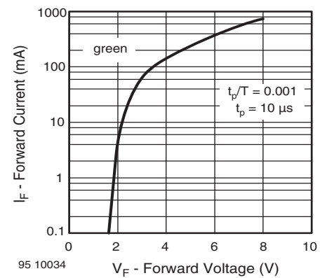
Fig. 18 - Forward Current vs. Forward Voltage
