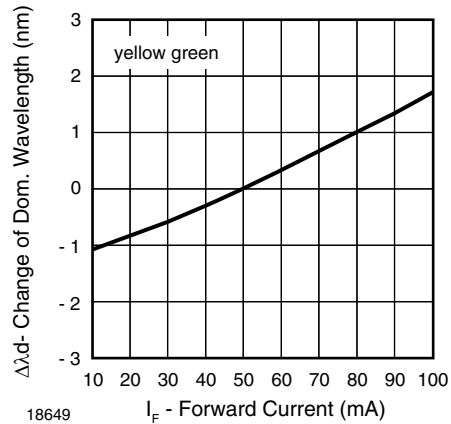
Fig. 30 - Change of Dominant Wavelength vs. Forward Current
