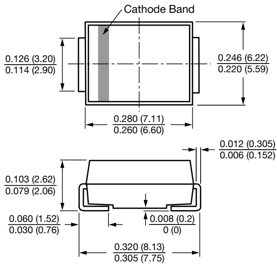
SMC (DO-214AB)
