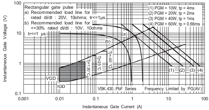
Fig. 12 - Gate Characteristics
