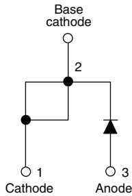
TO-247AC modified
