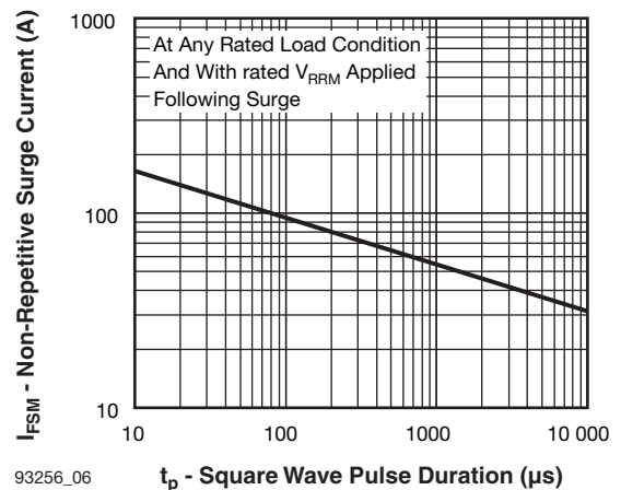
93256_06 Fig. 6 - Typical Non-Repetitive Surge Current
