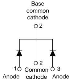
VS-MBR20..CT-1PbF
