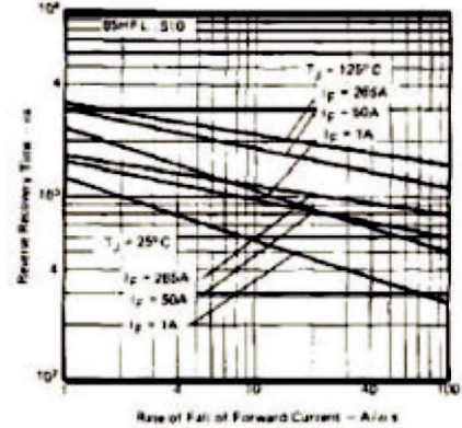
Fig. 35 - Typical Reverse Recovery Time vs. Rate of Fall of Forward Current, 85HFL...S10 Series
