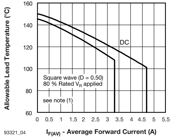
93321_04 I F(AV) - Average Forward Current (A) Fig. 4 - Maximum Allowable Lead Temperature vs. Average Forward Current
