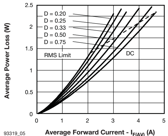
93319_05 Fig. 5 - Forward Power Loss Characteristics
