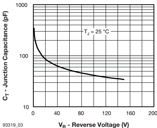
93319_03 Fig. 3 - Typical Junction Capacitance vs. Reverse Voltage
