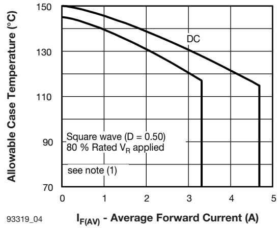
93319_04 Fig. 4 - Maximum Allowable Lead Temperature vs. Average Forward Current
