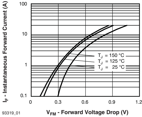
93319_01 Fig. 1 - Maximum Forward Voltage Drop Characteristics
