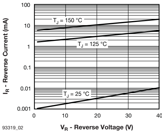
93319_02 Fig. 2 - Typical Values of Reverse Current vs. Reverse Voltage
