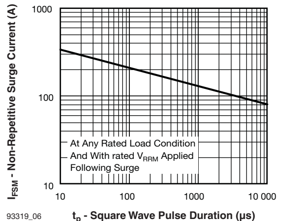
93319_06 Fig. 6 - Maximum Non-Repetitive Surge Current
