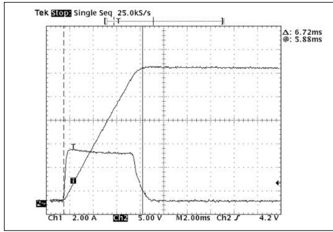
Figure 4— Inrush Limiting: Inrush current with 1000 \mu F external capacitance, (C1 in Figure 5)
