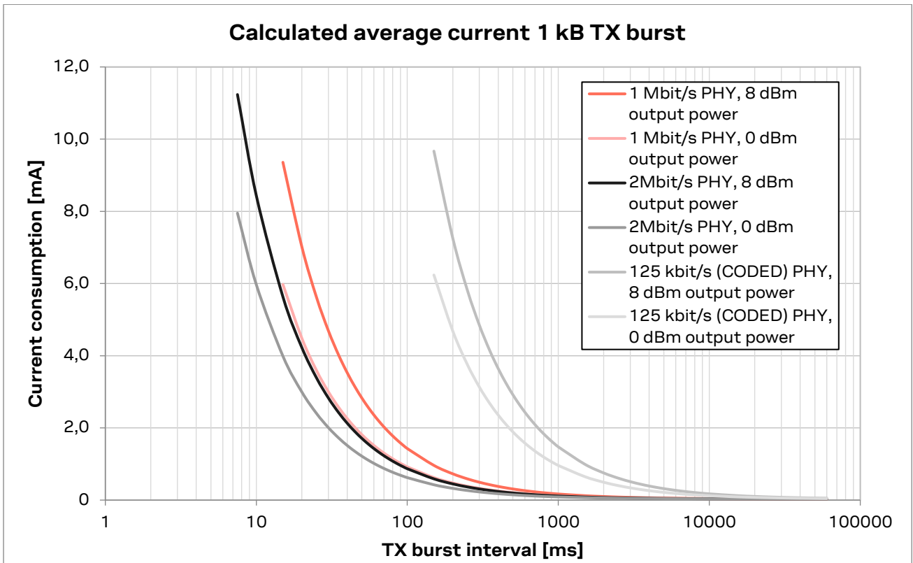
Figure 8: The average standby and TX current for different BLE PHY configurations when transmitting a 1 kB data packet at various intervals.
