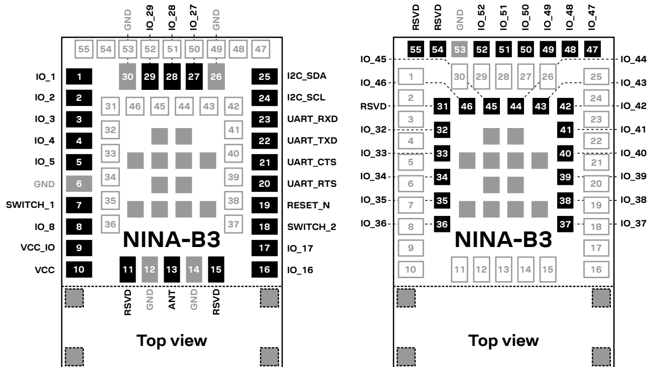
Figure 5: NINA-B31 JavaScript series pin assignment (top view)
