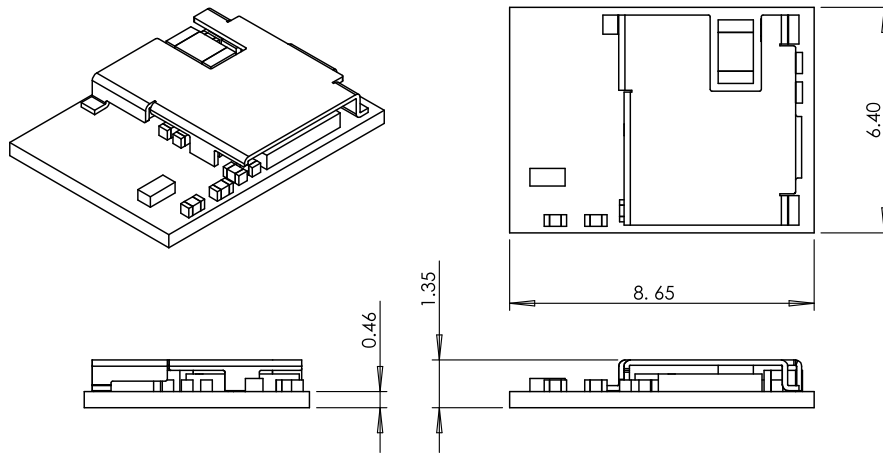
Figure 4 – Mechanical Drawing
