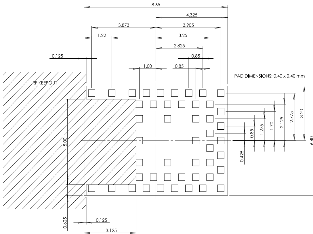
Figure 5 – Recommended PCB Land Pads
