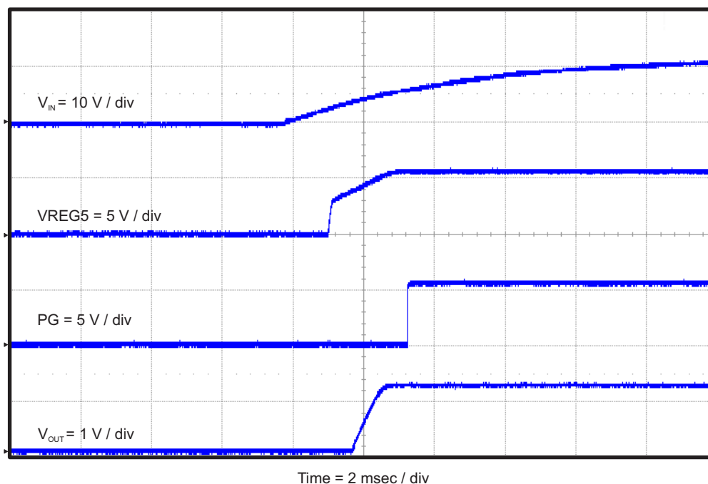
Figure 10. TPS56428EVM-534 Start-Up Relative to V_{IN} with VREG5, PG and V_{OUT}
