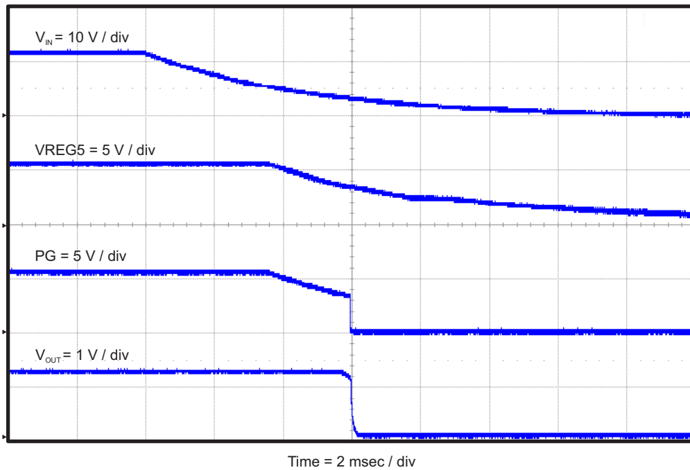
Figure 12. TPS56428EVM-534 Shut-Down Relative to V_{IN} with VREG5, PG and V_{OUT}
