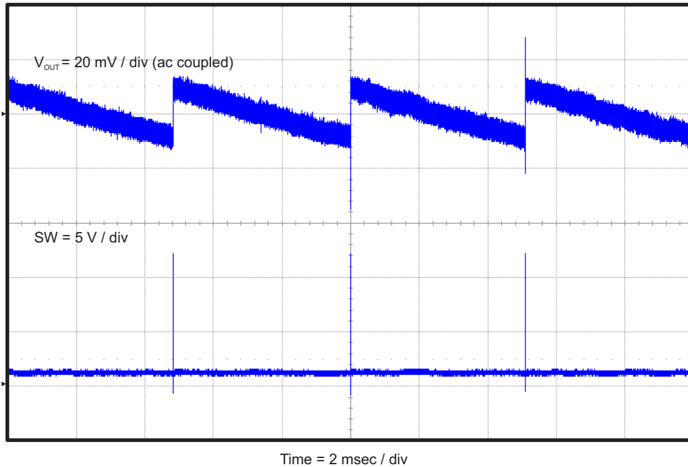
Figure 8. TPS56428EVM-534 Output Voltage Ripple ( I_{OUT} = 1 \text{ mA} )
