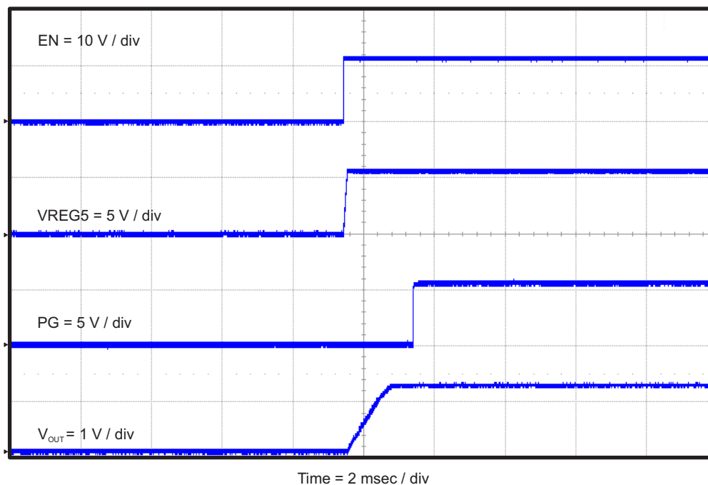
Figure 11. TPS56428EVM-534 Start-Up Relative to EN with VREG5, PG and V_{OUT}
