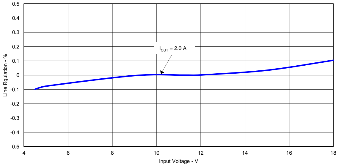
Figure 4. TPS56428EVM-534 Line Regulation
