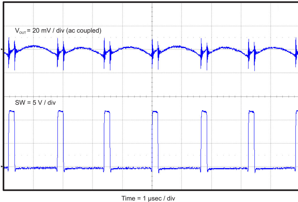
Figure 6. TPS56428EVM-534 Output Voltage Ripple ( I_{OUT} = 4 \text{ A} )
