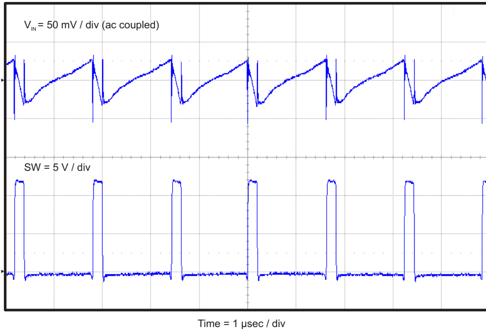
Figure 9. TPS56428EVM-534 Input Voltage Ripple
