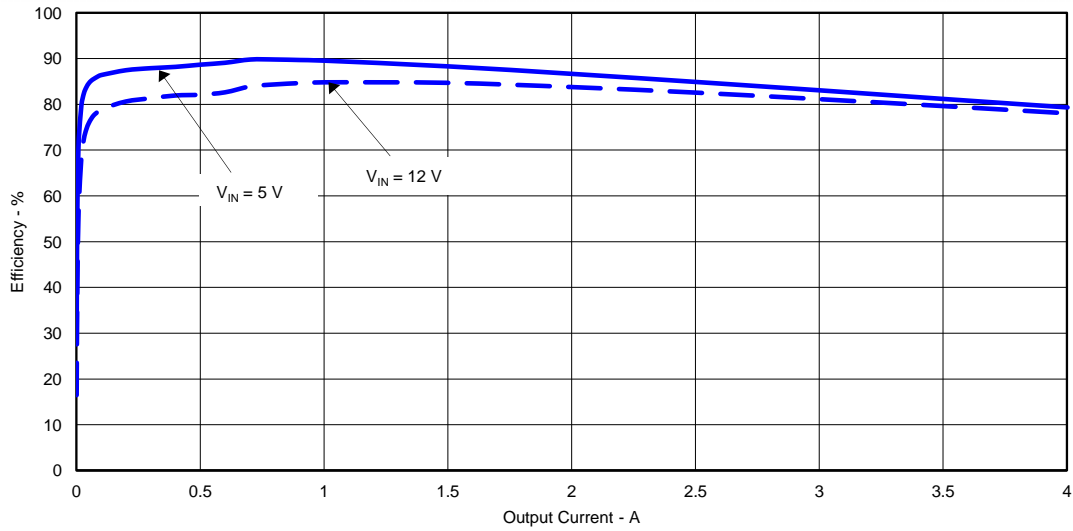
Figure 1. TPS56428EVM-534 Efficiency
