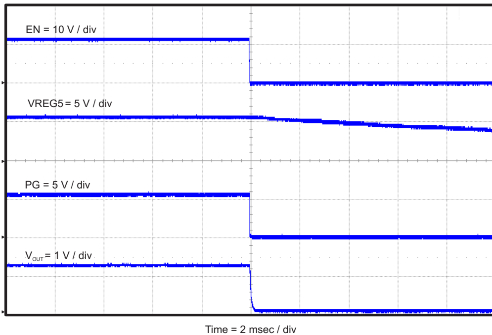
Figure 13. TPS56428EVM-534 Shut-Down Relative to EN with VREG5, PG and V_{OUT}
