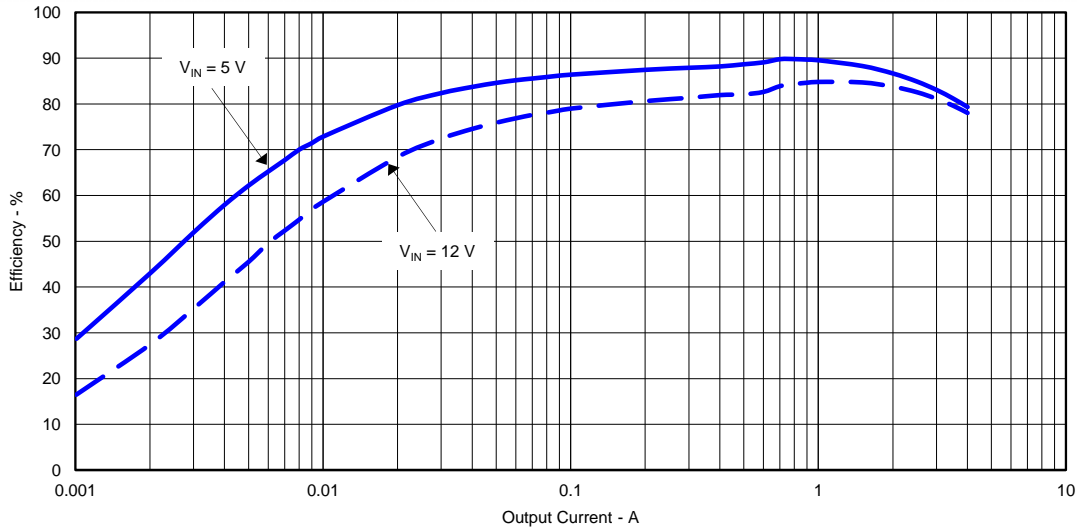
Figure 2. TPS56428EVM-534 Light-Load Efficiency
