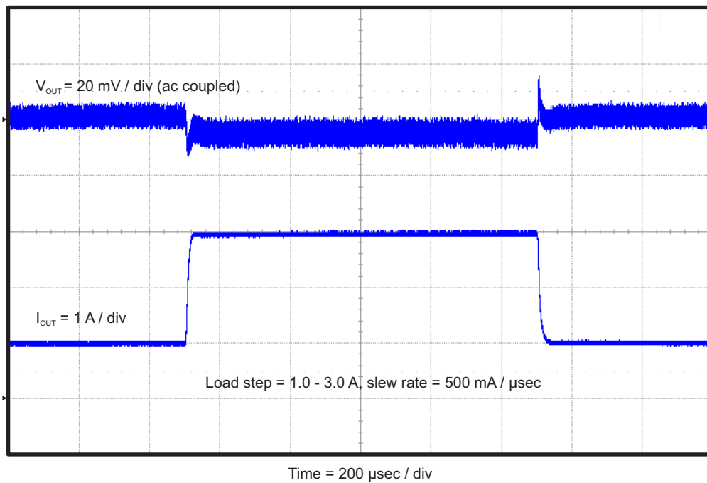
Figure 5. TPS56428EVM-534 Load Transient Response
