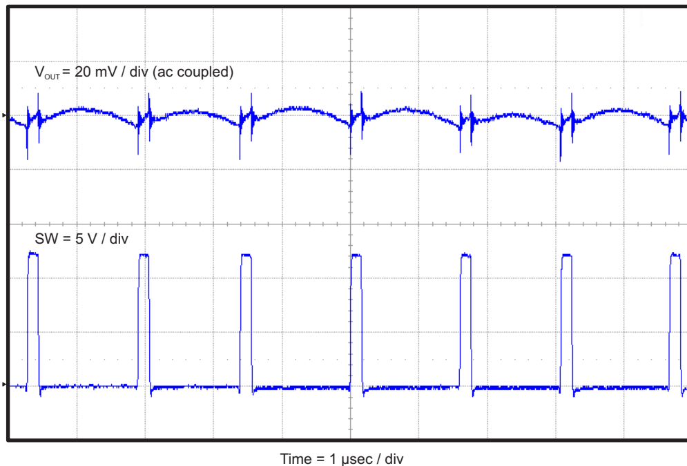
Figure 7. TPS56428EVM-534 Output Voltage Ripple ( I_{OUT} = 500 \text{ mA} )
