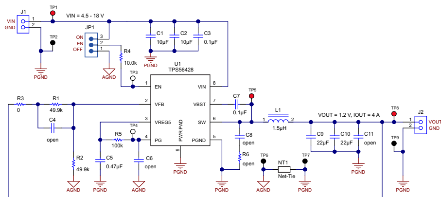
Figure 19. TPS56428EVM-534 Schematic Diagram
