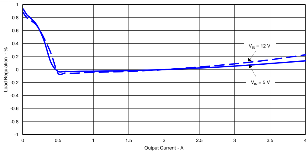
Figure 3. TPS56428EVM-534 Load Regulation, V_{IN} = 5\text{ V} and V_{IN} = 12\text{ V}
