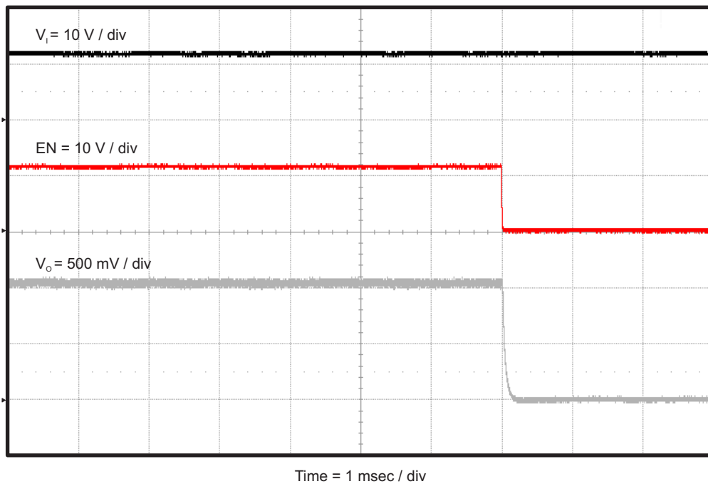
Figure 13. TPS563209EVM-652 Shut-Down Relative to EN
