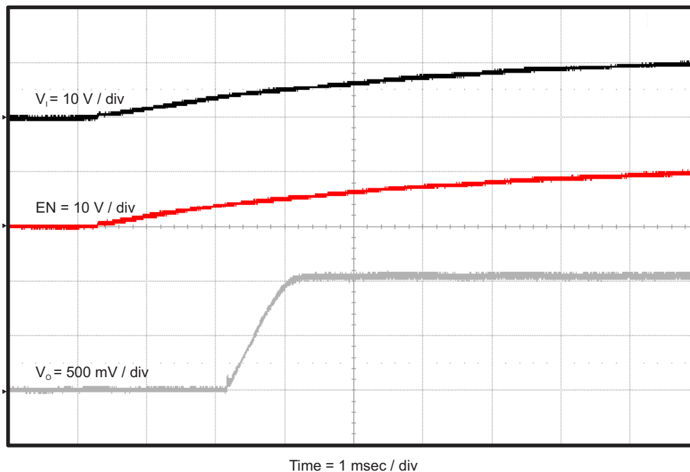
Figure 10. TPS563209EVM-652 Start-Up Relative to V_{IN}
