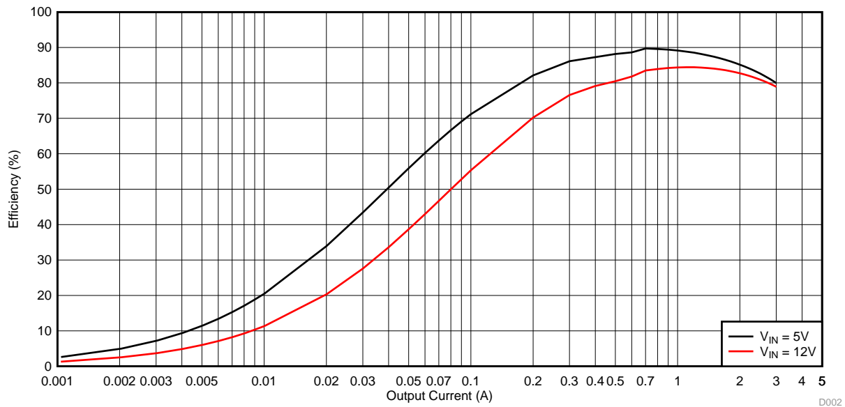
Figure 2. TPS563209EVM-652 Light Load Efficiency
