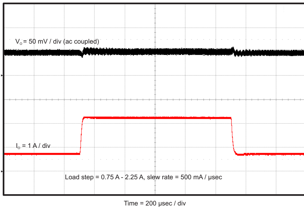
Figure 6. TPS563209EVM-652 Load Transient Response, 25% to 75% Load Step
