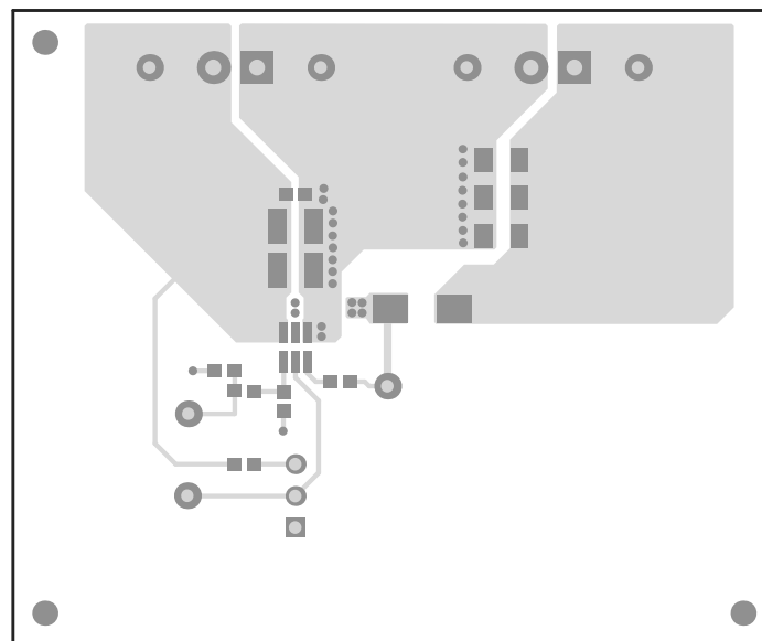
Figure 15. Top Layer
