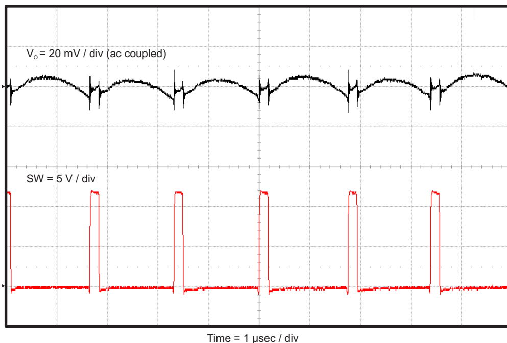
Figure 7. TPS563209EVM-652 Output Voltage Ripple, I_{OUT} = 3\text{ A}
