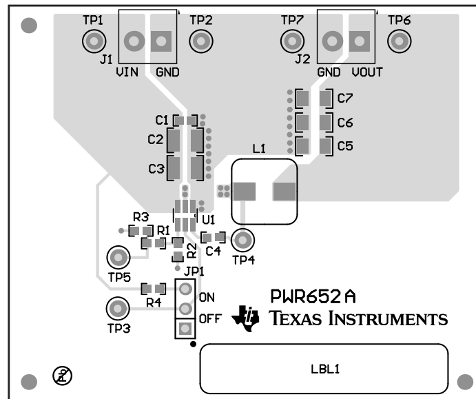
Figure 14. Top Assembly
