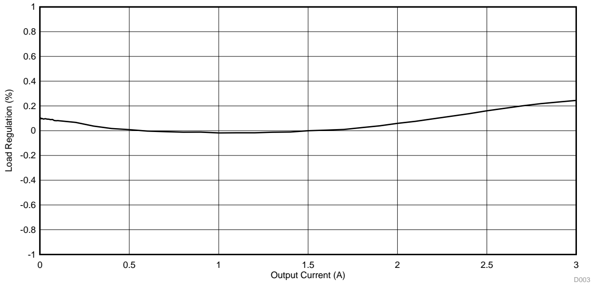
Figure 3. TPS563209EVM-652 Load Regulation, 5-V Input
