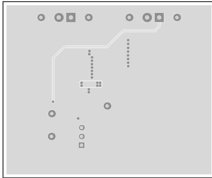
Figure 16. Bottom Layer
