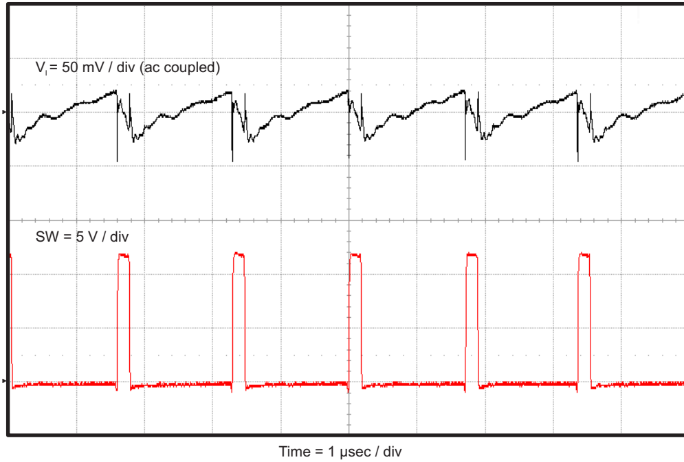
Figure 9. TPS563209EVM-652 Input Voltage Ripple, I_{\text{OUT}} = 3 \text{ A}
