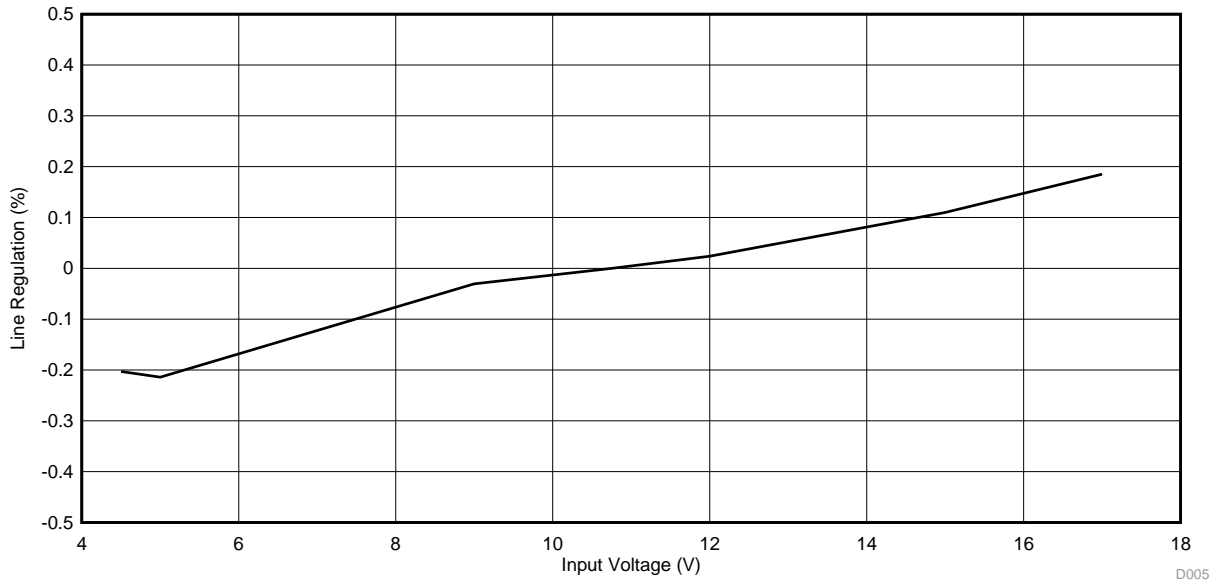
Figure 5. TPS563209EVM-652 Line Regulation
