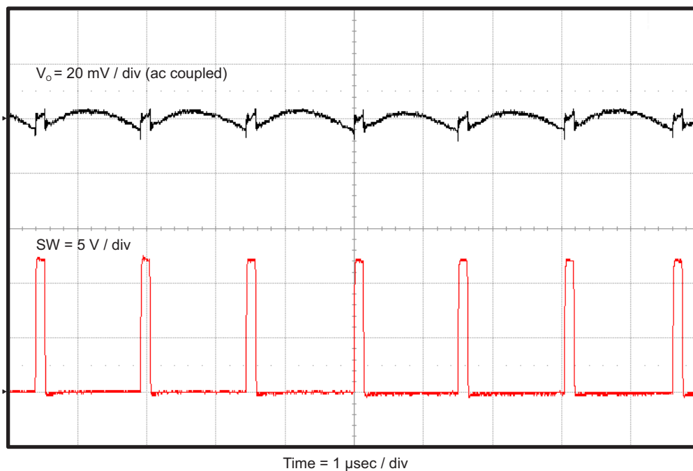
Figure 8. TPS563209EVM-652 Output Voltage Ripple, I_{OUT} = 0\text{ mA}
