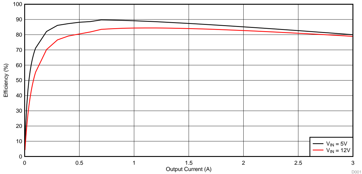
Figure 1. TPS563209EVM-652 Efficiency
