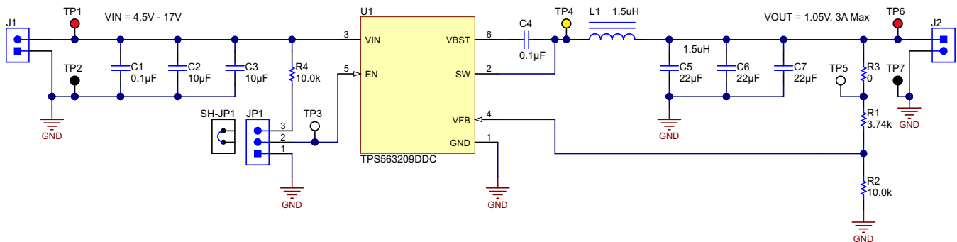
Figure 17. TPS563209EVM-652 Schematic Diagram
