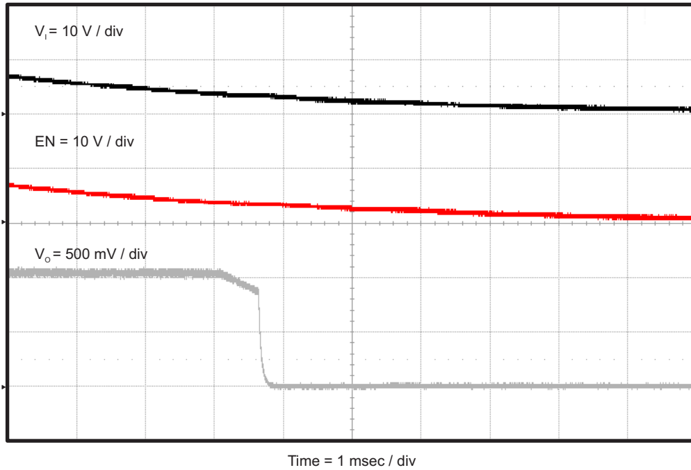
Figure 12. TPS563209EVM-652 Shut-Down Relative to V_{IN}
