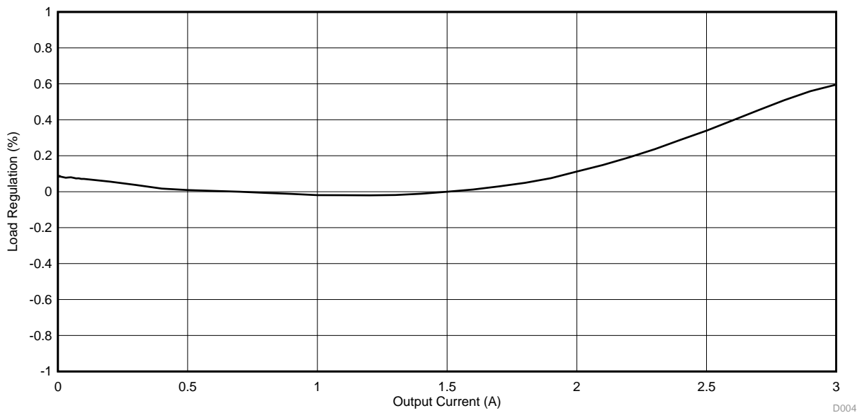
Figure 4. TPS563209EVM-652 Load Regulation, 12-V Input
