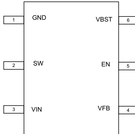
TPS562200, TPS563200 DDC (SOT) Package Top View
