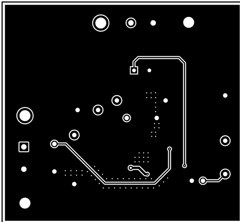
Figure 8. Bottom Layer
