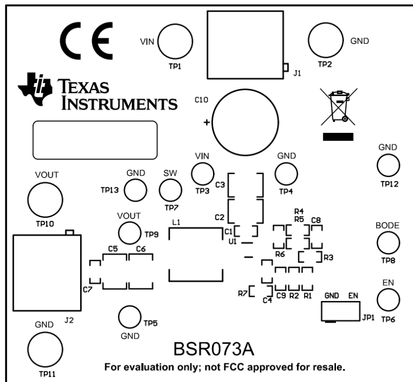
Figure 6. Top Assembly
