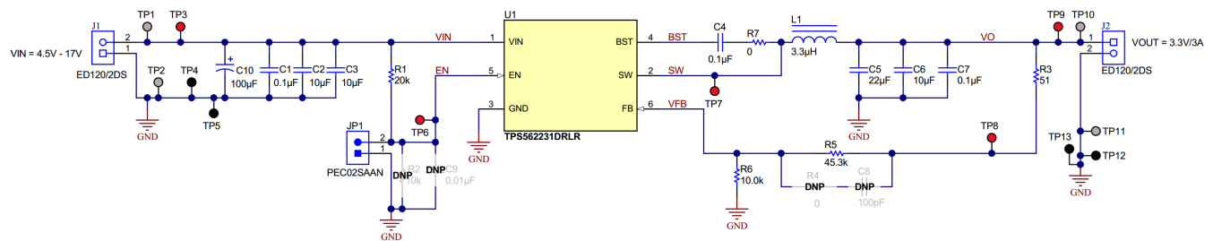
Figure 9. TPS562231EVM Schematic Diagram
