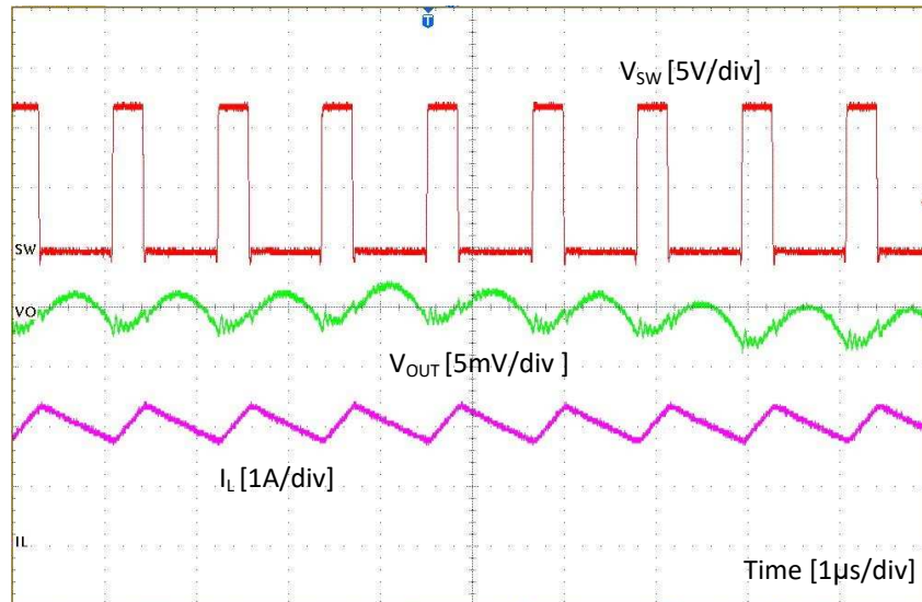
Figure 3. TPS562231EVM Output Voltage Ripple in CCM
