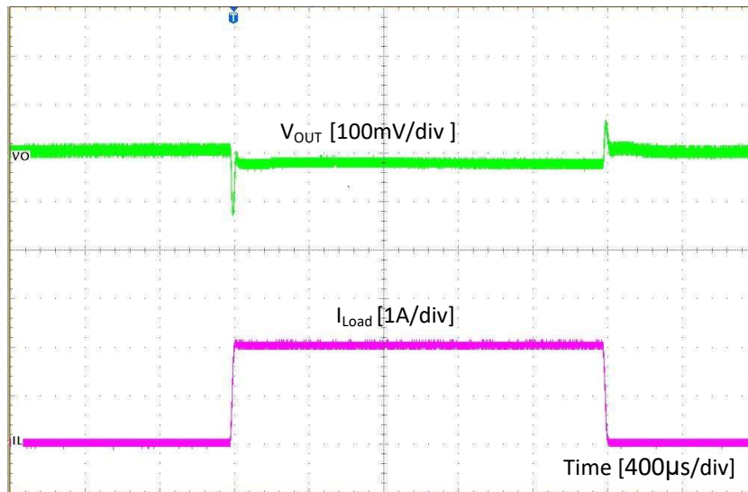
Figure 2. TPS562231EVM Load Transient Response
