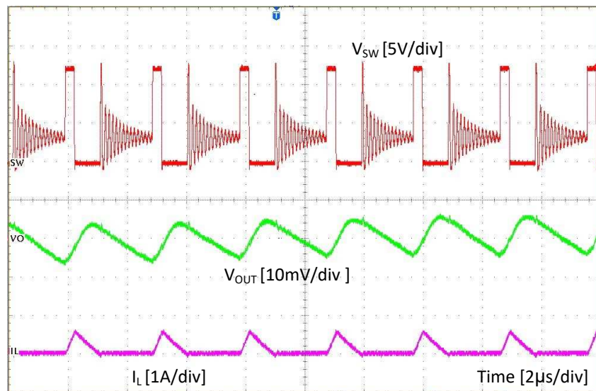
Figure 4. TPS562231EVM Output Voltage Ripple in DCM
