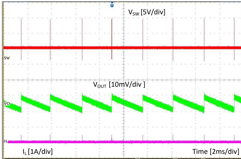
Figure 5. TPS562231EVM Output Voltage Ripple on No-load
