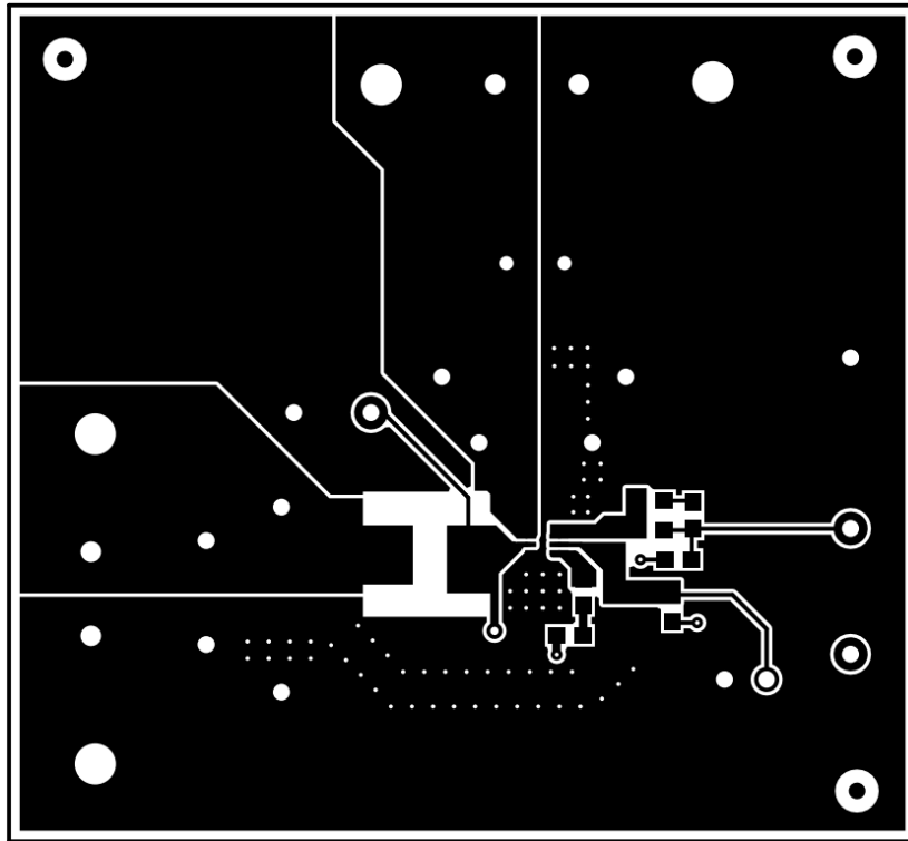
Figure 7. Top Layer
