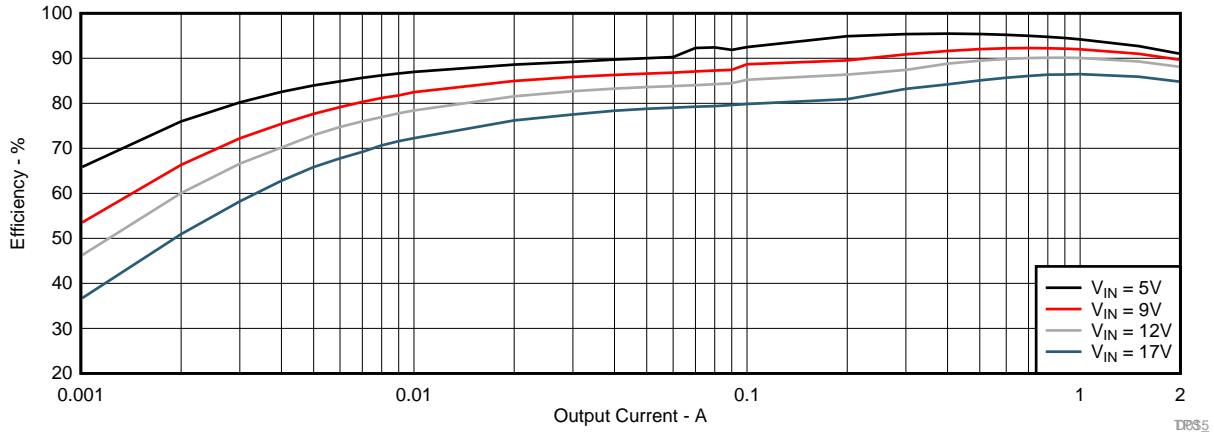
Figure 1. TPS562231EVM Efficiency
