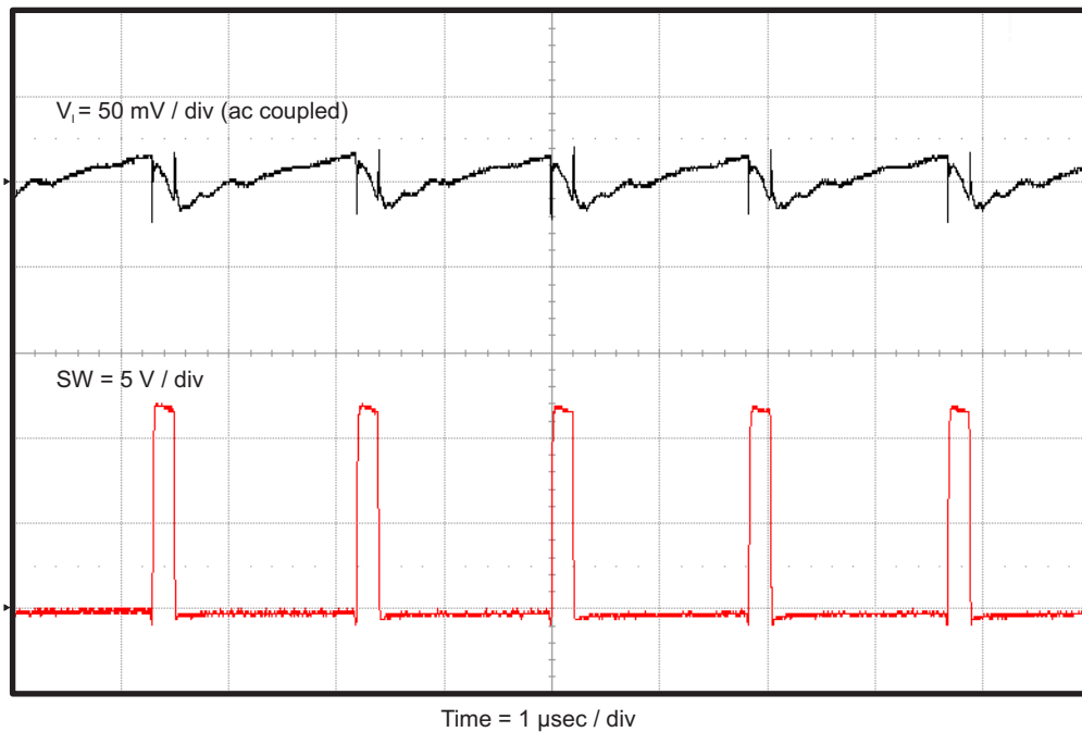
Figure 8. TPS562219EVM-663 Input Voltage Ripple, I_{OUT} = 2 \text{ A}
