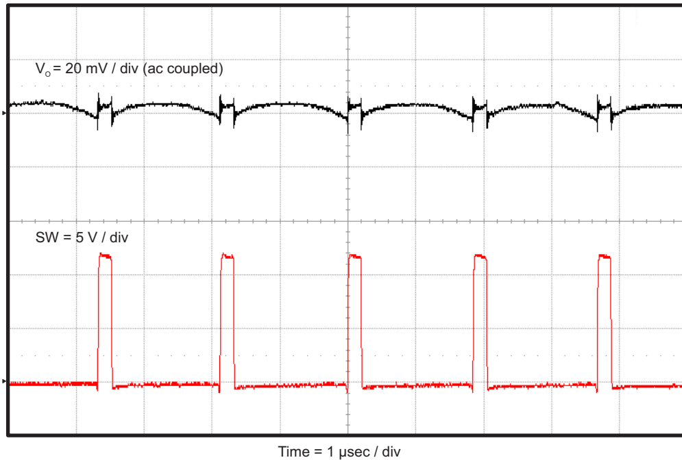
Figure 7. TPS562219EVM-663 Output Voltage Ripple, I_{OUT} = 2 \text{ A}
