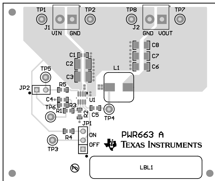
Figure 13. Top Assembly
