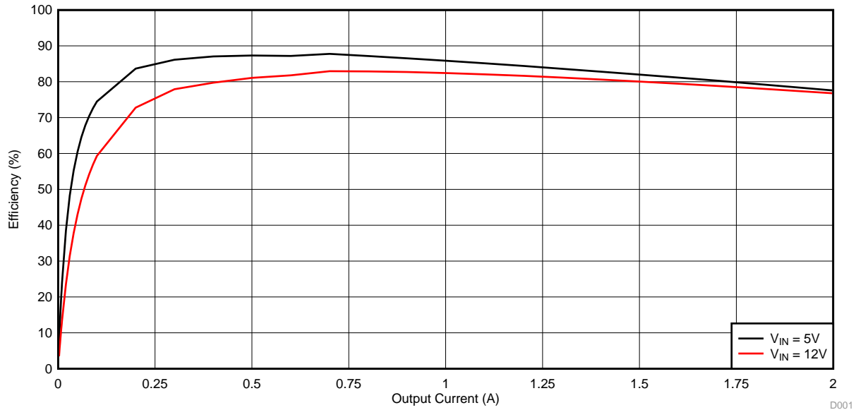
Figure 1. TPS562219EVM-663 Efficiency
