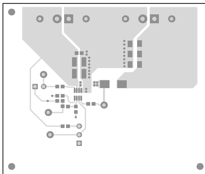
Figure 14. Top Layer
