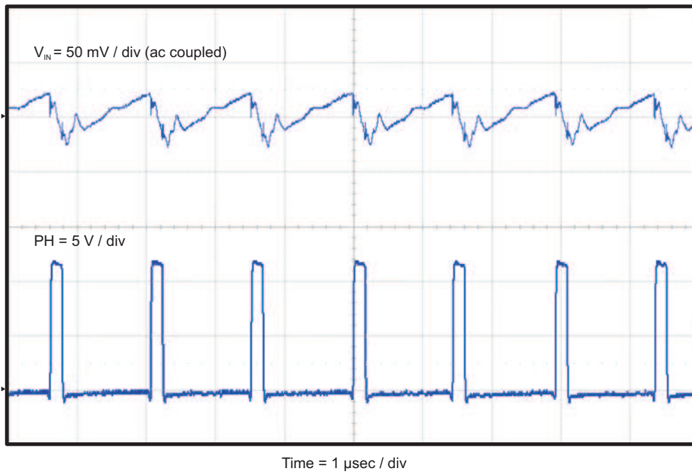
Figure 10. TPS54329EEVM-056 Input Voltage Ripple
