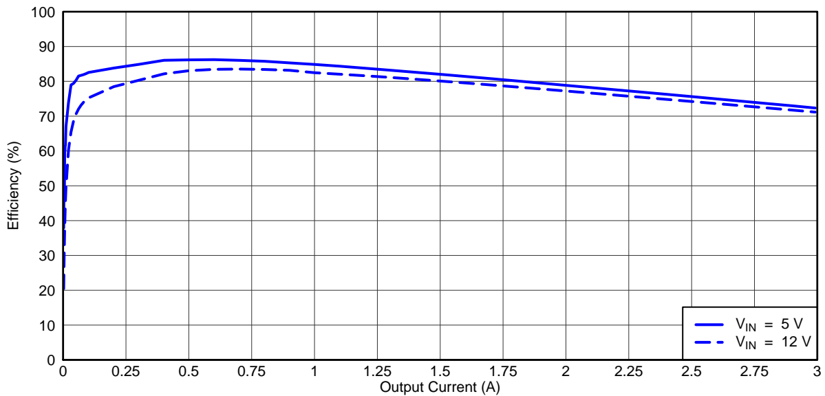
Figure 1. TPS54329EEVM-056 Efficiency
