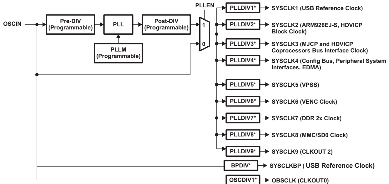
Figure 3-3. PLLC1 Configuration
