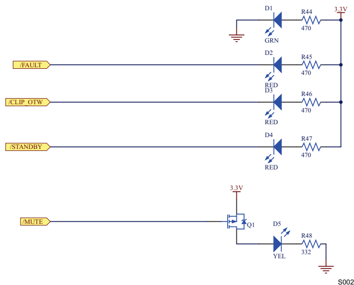
Figure 7. TAS5412-Q1 EVM Schematic (Sheet 2 of 2)
