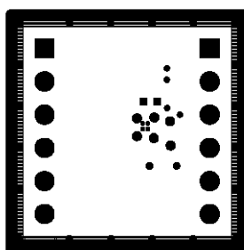
Figure 9. SMP-TPS7A4901-MVK Board Solder Mask – Bottom Side
