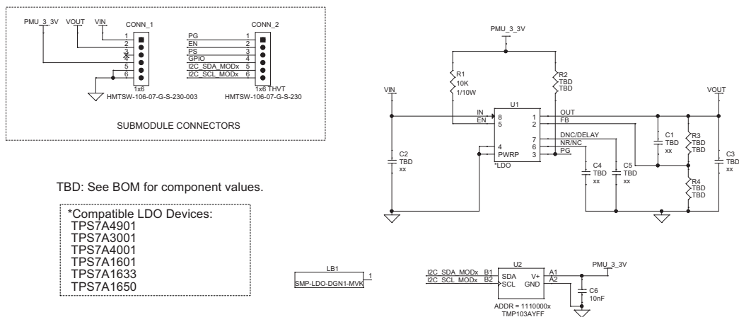
Figure 14. SMP-TPS7A4901-MVK Schematic
