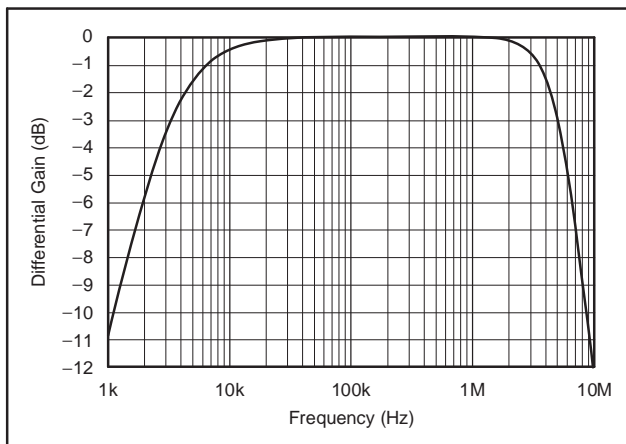
Figure 68. 5MHz, 2nd-Order, Butterworth Low-Pass Filter
