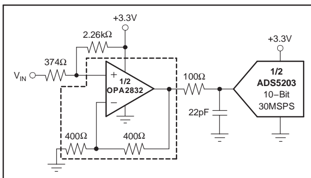
Figure 64. DC-Coupled, +3V ADC Driver
