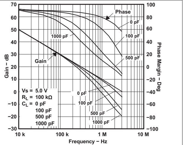
Figure 4. LMV321 Frequency Response vs Capacitive Load
