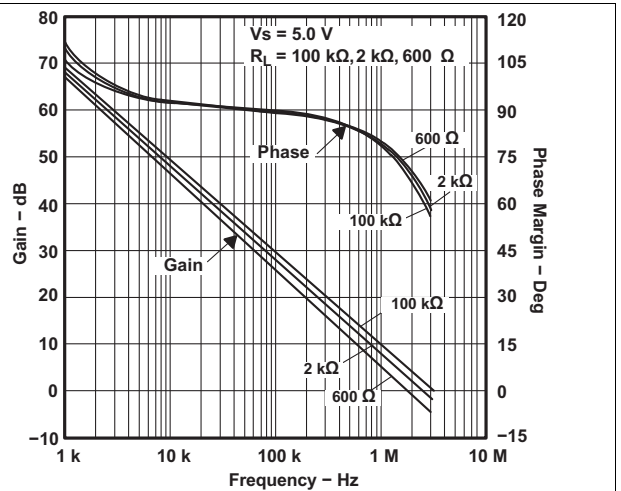
Figure 2. LMV321 Frequency Response vs Resistive Load
