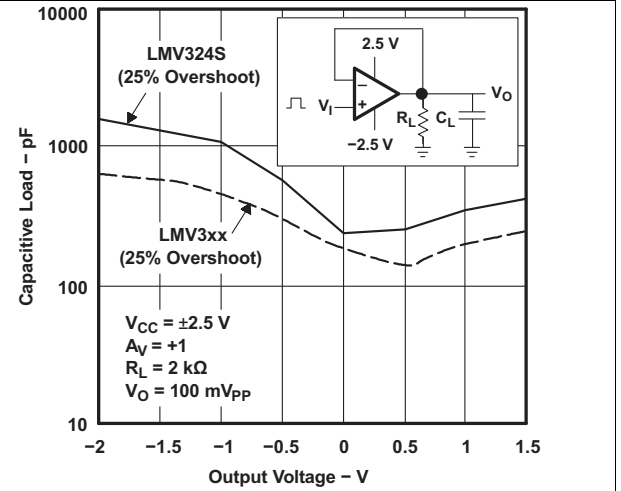
Figure 6. Stability vs Capacitive Load
