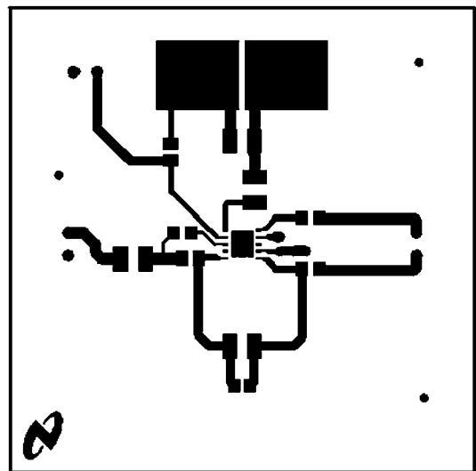
FIGURE 3. Recommended TS SE PCB Layout: Top Layer
