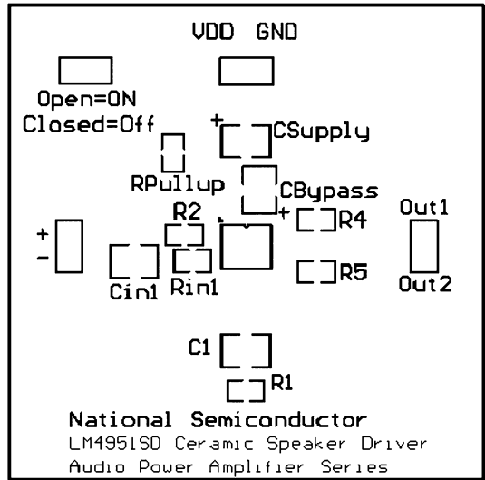
FIGURE 2. Recommended TS SE PCB Layout: Top Silkscreen
