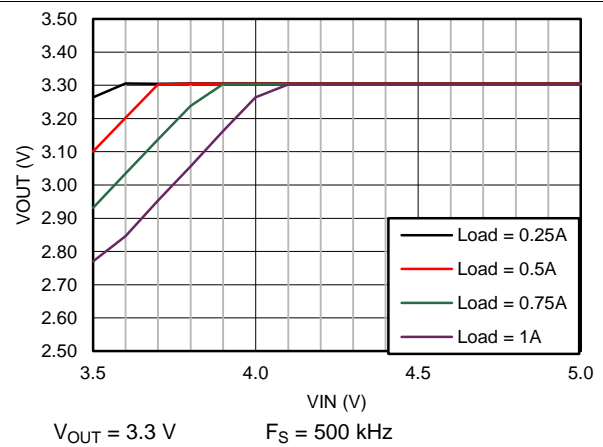
Figure 50. Drop-Out Curve
