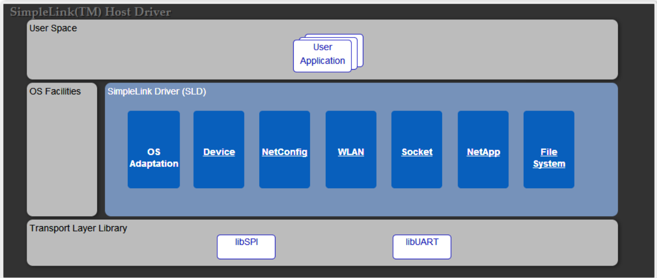
Figure 1-2. Host Driver Anatomy
