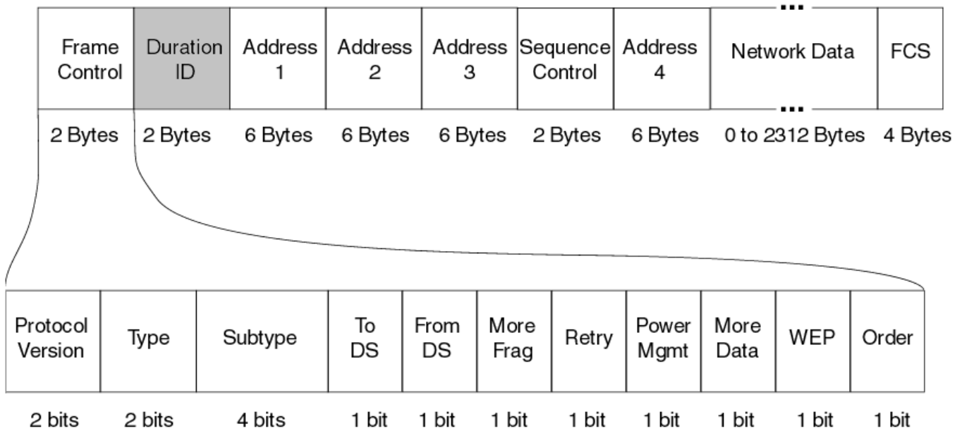
Figure 16-1. 802.11 Frame Structure
