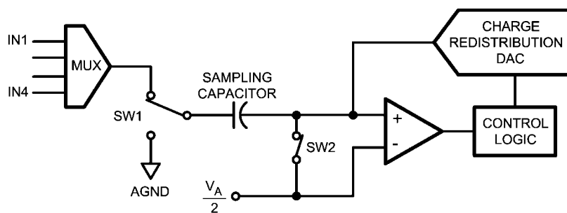
FIGURE 1. ADC124S021 in Track Mode
