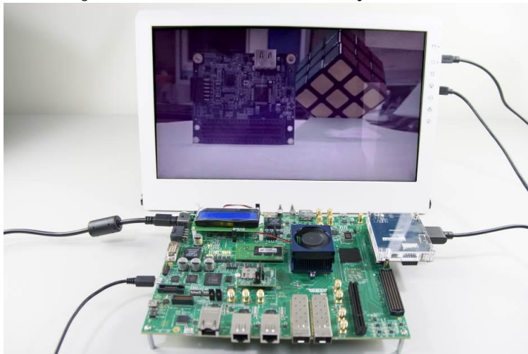
Figure 5-10 A10SoC_D8M_FMC_VIP demonstration running on A10SoC
