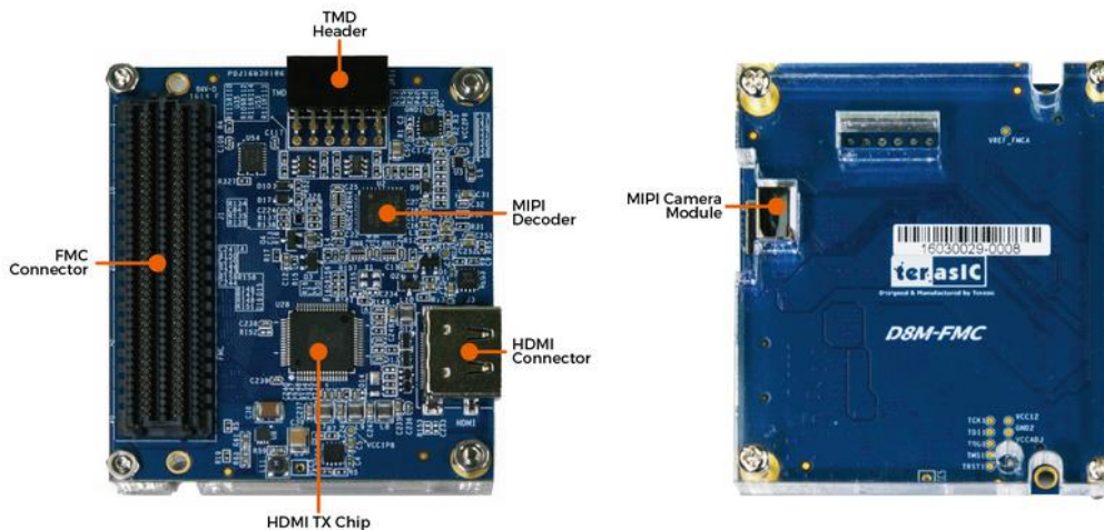
Figure 2-1 D8M-FMC Board
