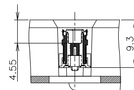
SECT. E-E (SCALE 2:1)
