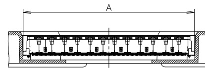
SECT. D-D (SCALE 2:1) (CONNECTOR NOT SECTION)
