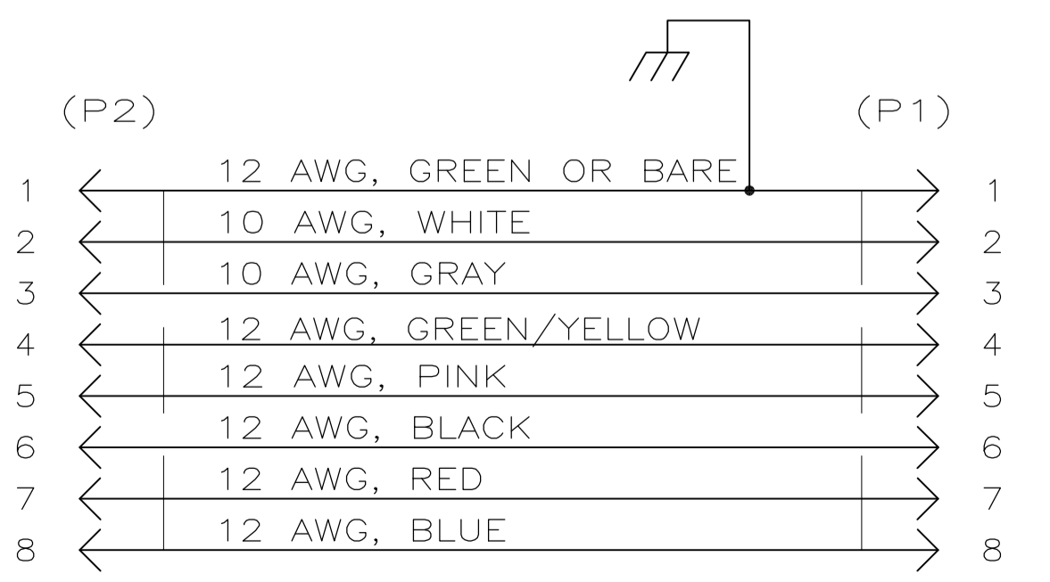
WIRING DIAGRAM 8 WIRE
