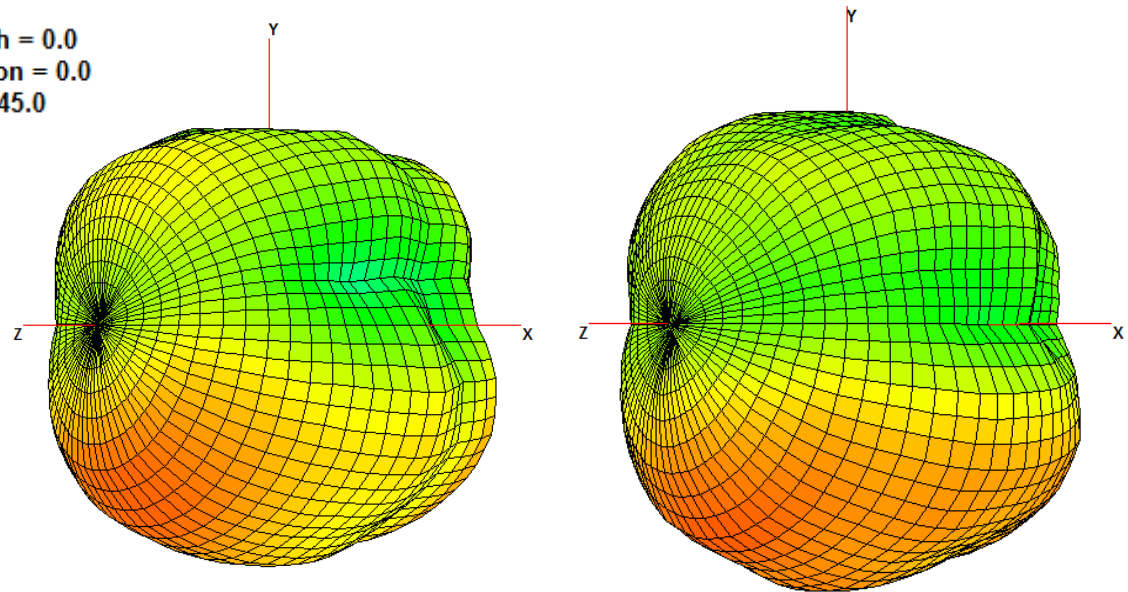
Figure 13. 3D Radiation Pattern at 1805 and 1910 MHz of the Warrior PA.711.A Antenna on MIMO PAD.71X.A
