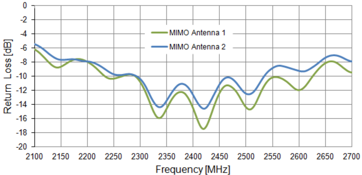
Figure 3. Return loss of the Hercules MA515 MIMO antenna from 2100 MHz to 2700 MHz.
