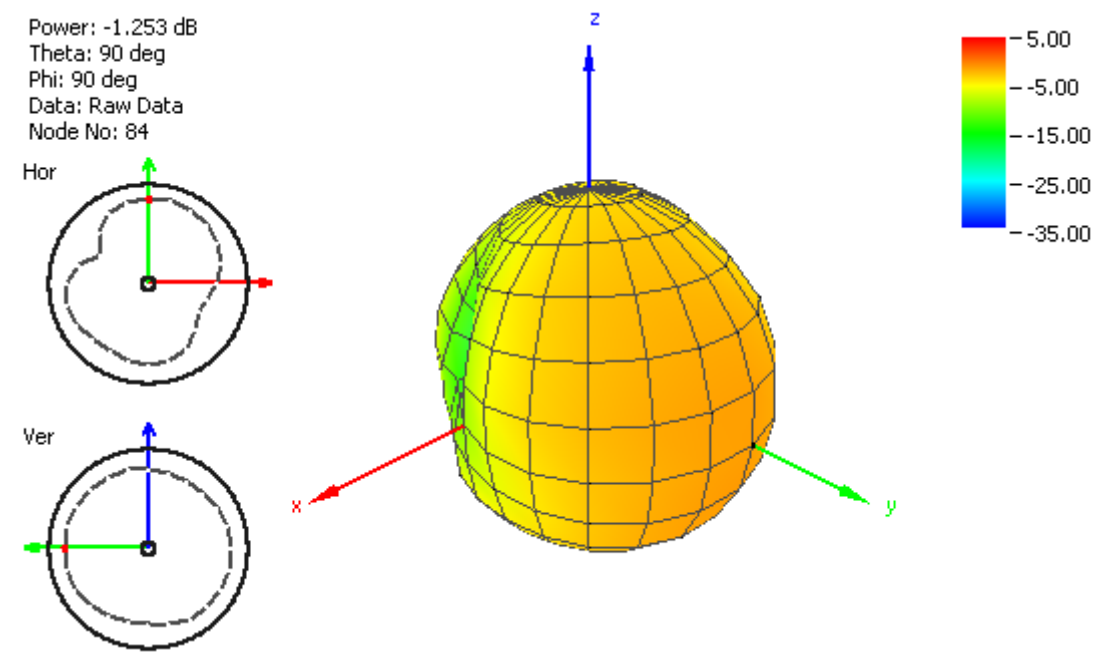
Figure 5. Radiation Pattern at 925 MHz.
