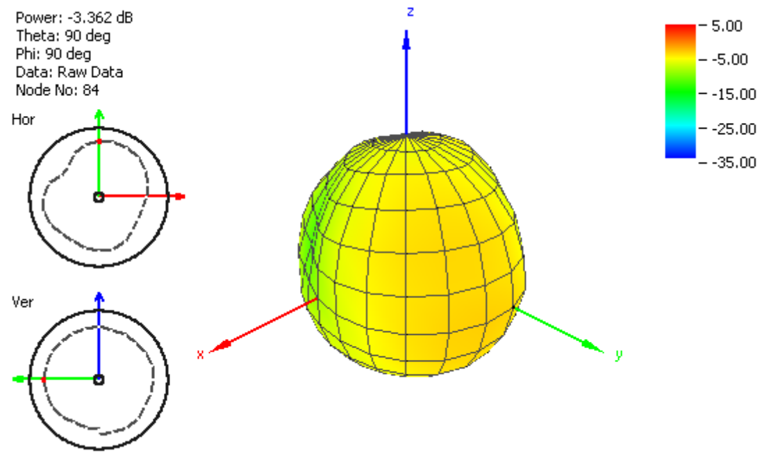
Figure 4. Radiation Pattern at 849 MHz.
