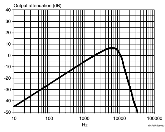
Figure 21. ITU R-ARM frequency response, weighting filter for transient pop
